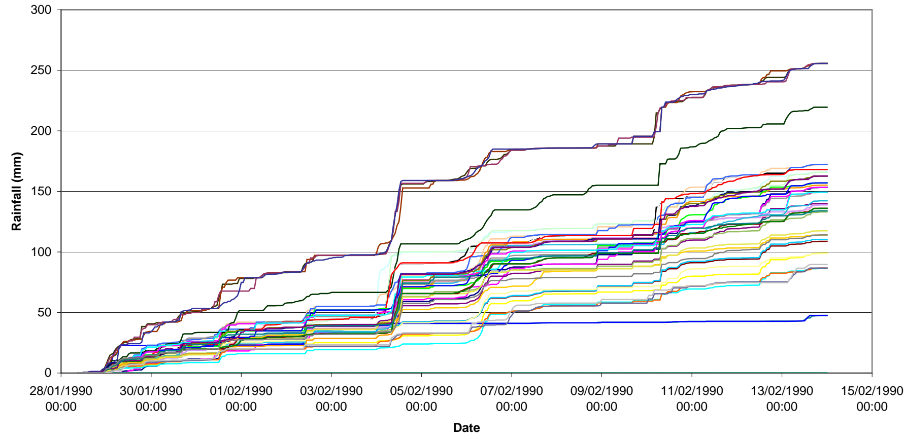
Cumulative rainfall profile 1990 event
