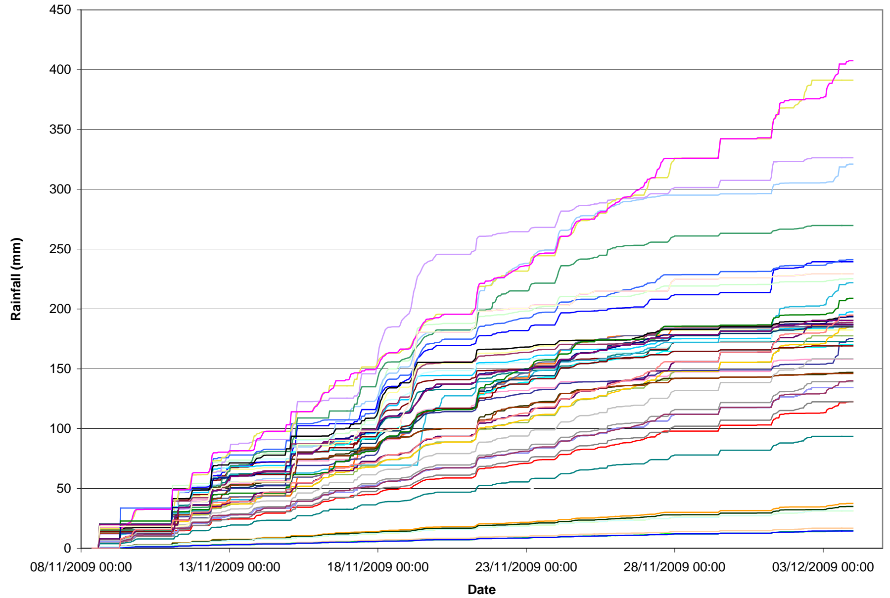
Cumulative rainfall profile 2009 event
