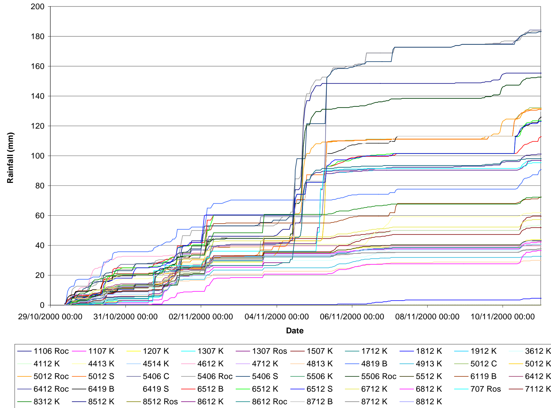
Cumulative rainfall profile 2000 event
